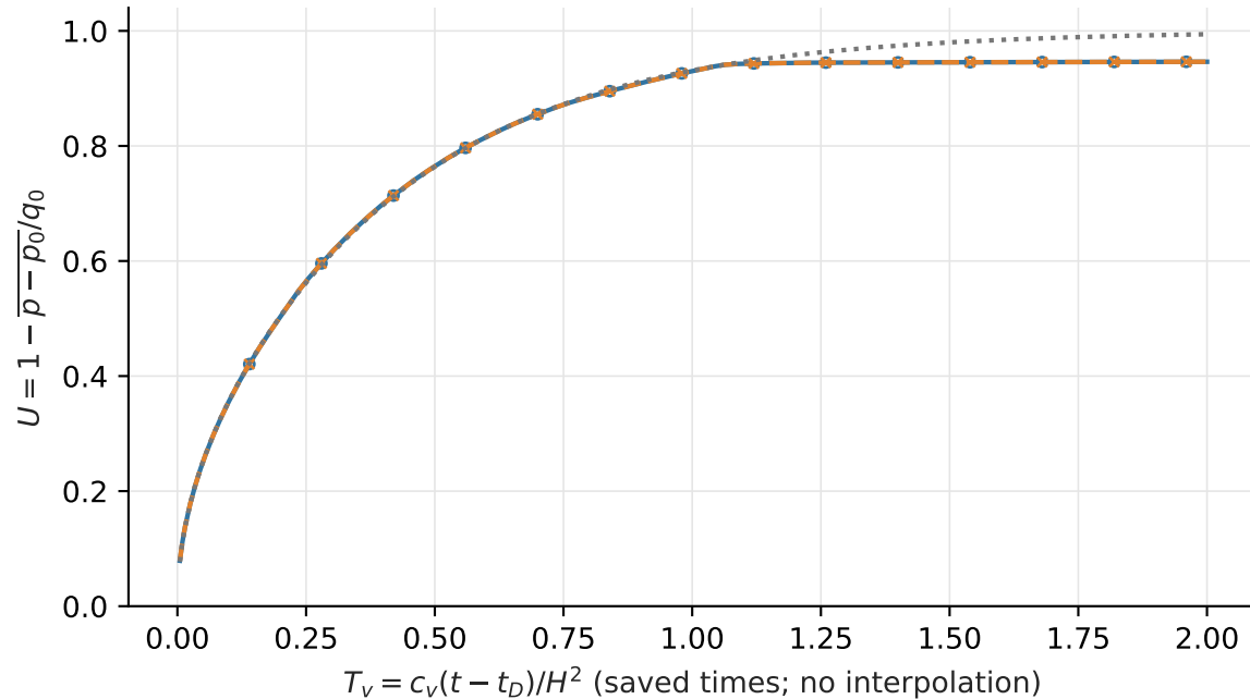
Pressure-based consolidation degree
