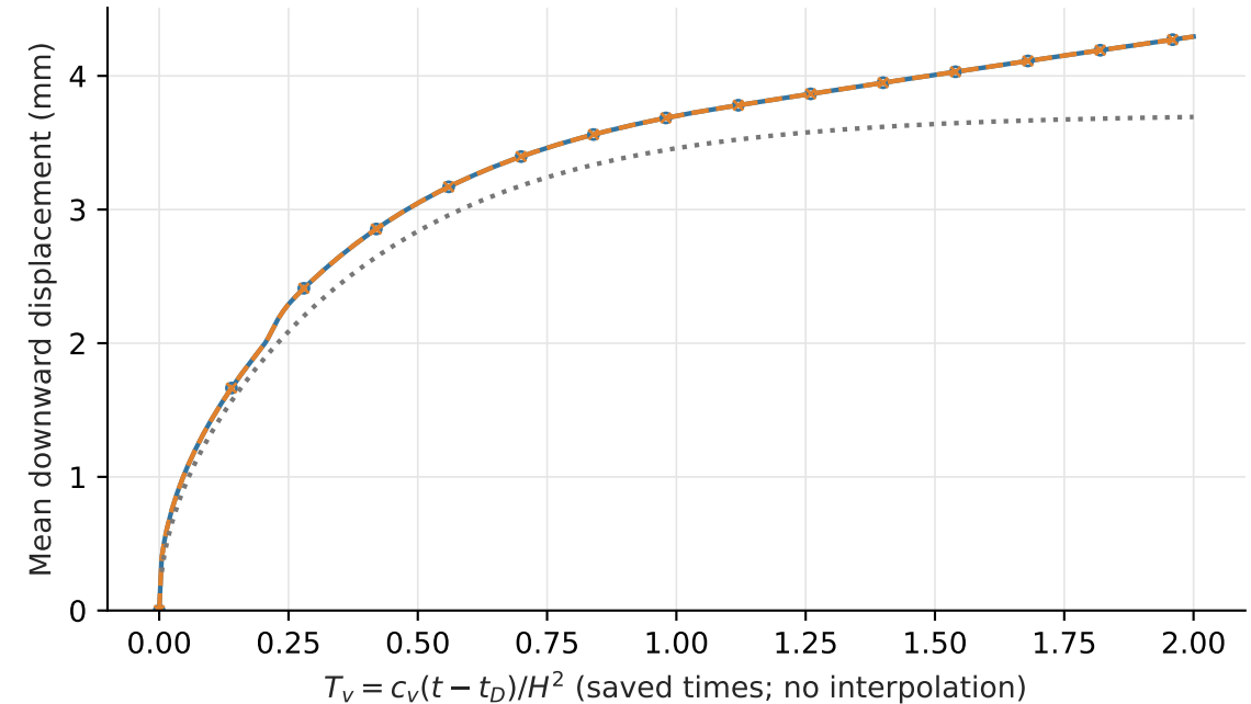
Settlement of fixed initial top IDs
