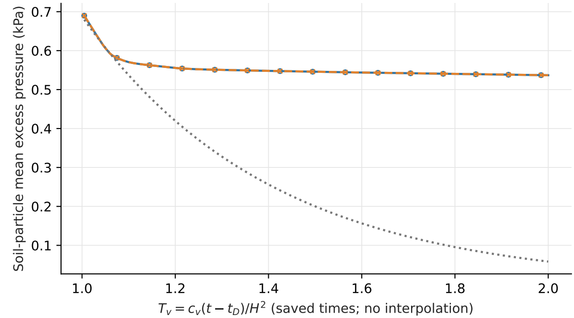
Late mean excess pressure ( T_v \geq 1 ; focused view)
