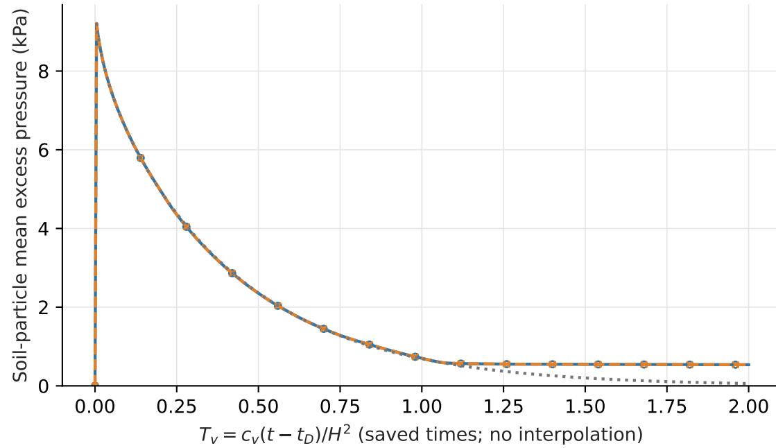
Mean excess pore pressure
